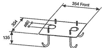
Anchorage plate 354x304 with M14x200 log bolts
