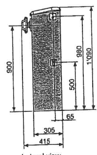
Lateral view photoelectric cell side
