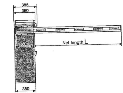
View with R532 arm connection on left-handed Bayt 980
