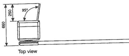
View with R532 arm connection on left-handed Bayt 980
